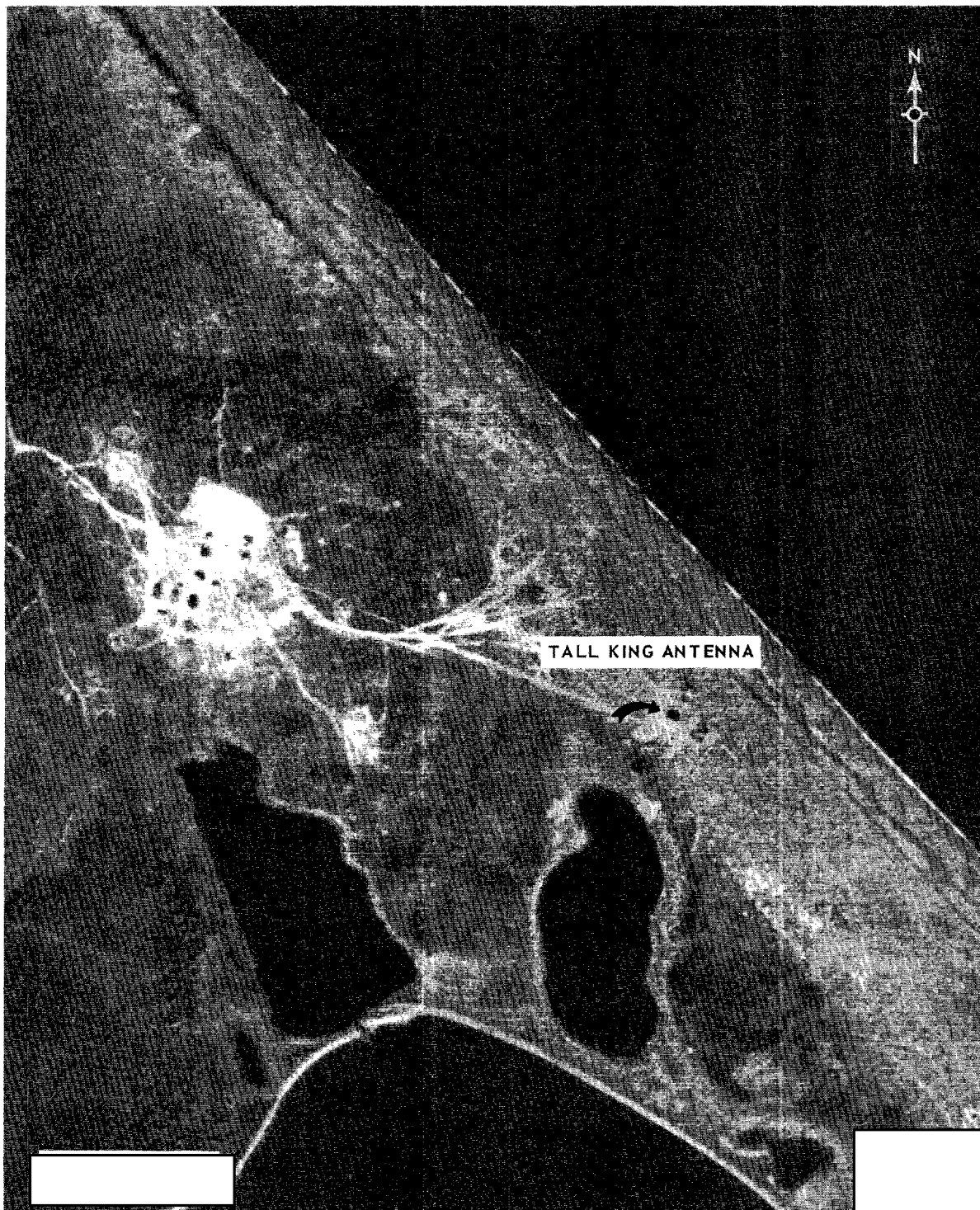
Ostrov Bolshoy Shantar TALL KING-AW Radar Facility
