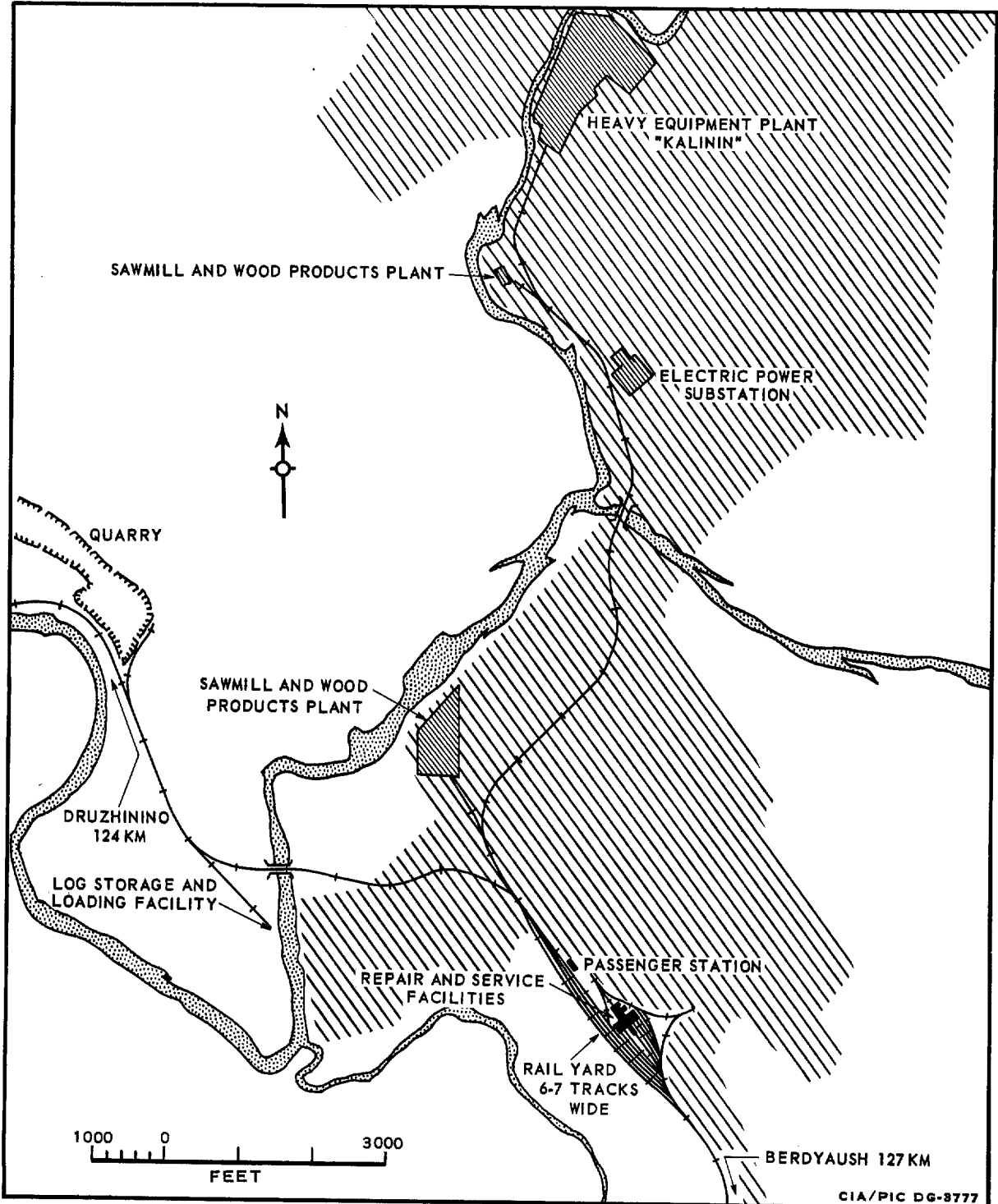
RAIL FACILITIES AT NYAZEPETROVSK, USSR
