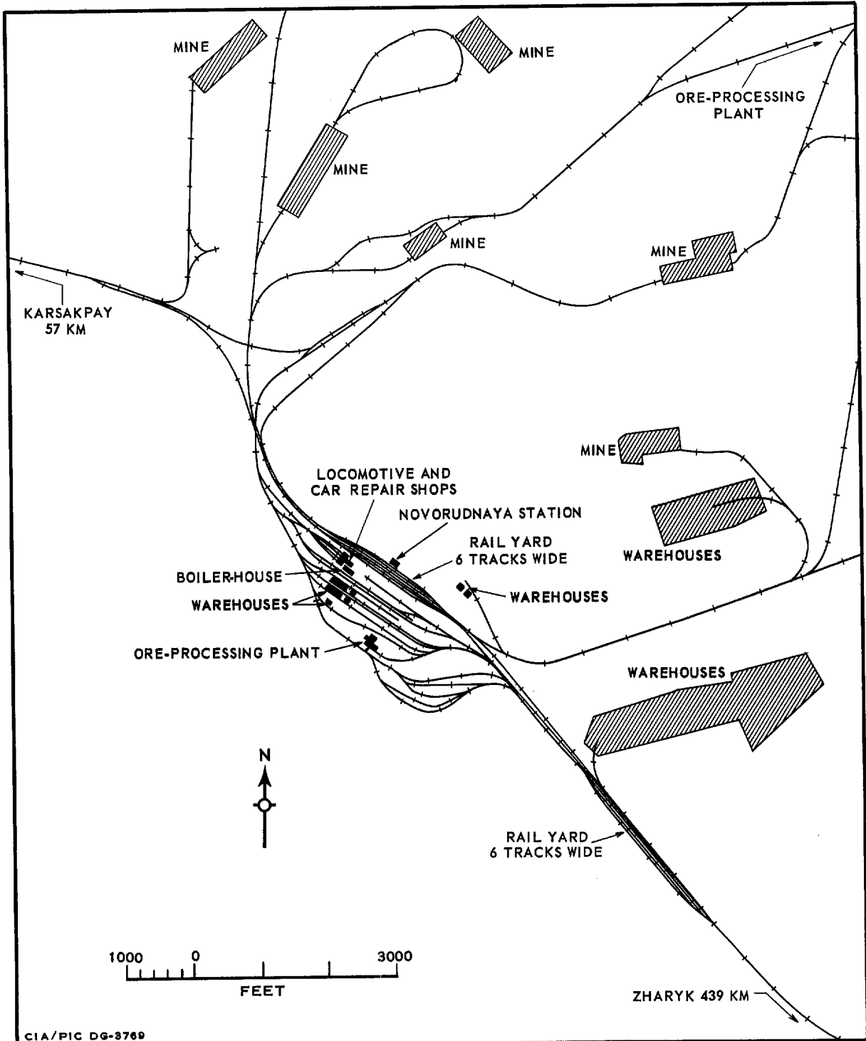
RAIL FACILITIES AT DZHEZKAZGAN, USSR
