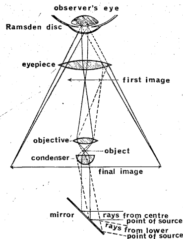
Fig. 1. Diagram illustrating the opinion that the eye of the microscopist is focused for close vision. (From Marshall and Griffith (1928). Reproduced by permission of Messrs. George Routledge and Sons Ltd. New lettering has been provided.)
