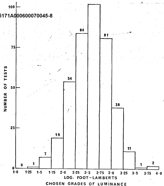
Fig. 11. Histogram showing the grades of luminance chosen by subjects in the tests of visual acuity. (The luminance is that of the ground glass plate placed 4 mm behind the test-object.)
