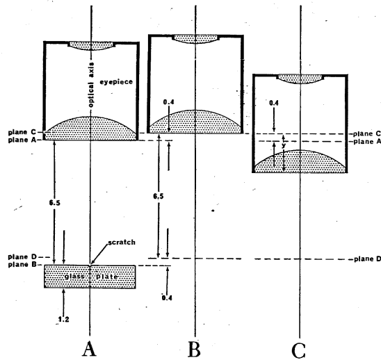
Fig. 3. Diagram illustrating, in greater detail than fig. 2, the author's method for determining the focus of the eye in microscopy by finding the distance y. The diagram is not drawn to scale; the numbers represent distances in millimetres.
