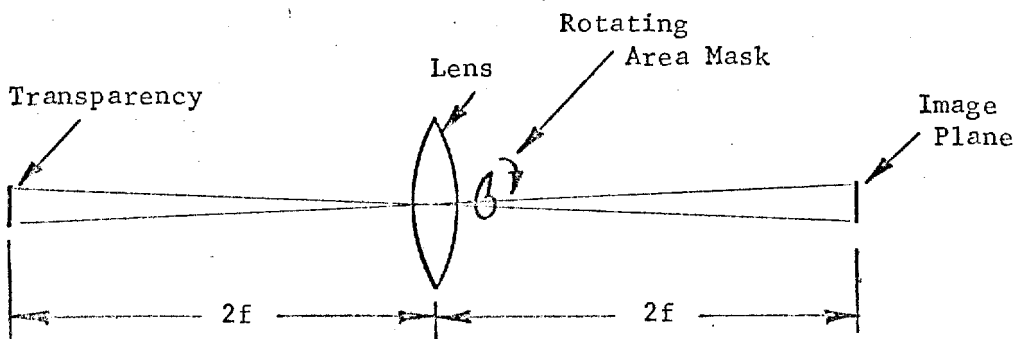
Figure 3. Modified Copy System
