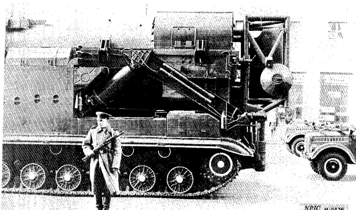
FIGURE 2. DETAIL OF REAR PORTION OF SCAMP TRANSPORTERS, MOSKVA PARADES, MAY 1967 (TOP) AND NOVEMBER 1966 (BOTTOM).
