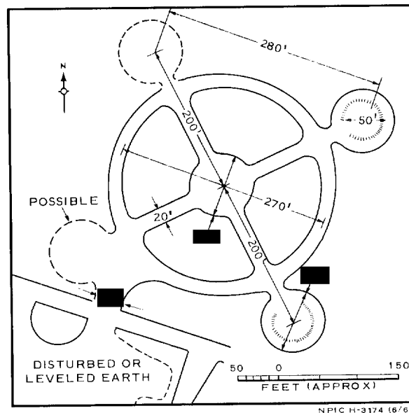
FIGURE 2. LAYOUT OF TRAINING SITE.
