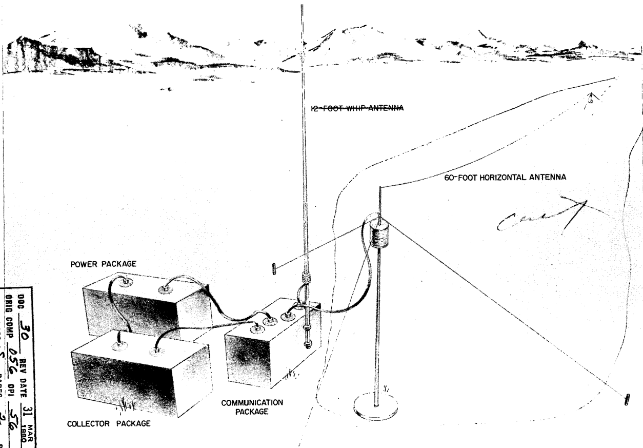
Figure 5-1. Field Unit configuration.
