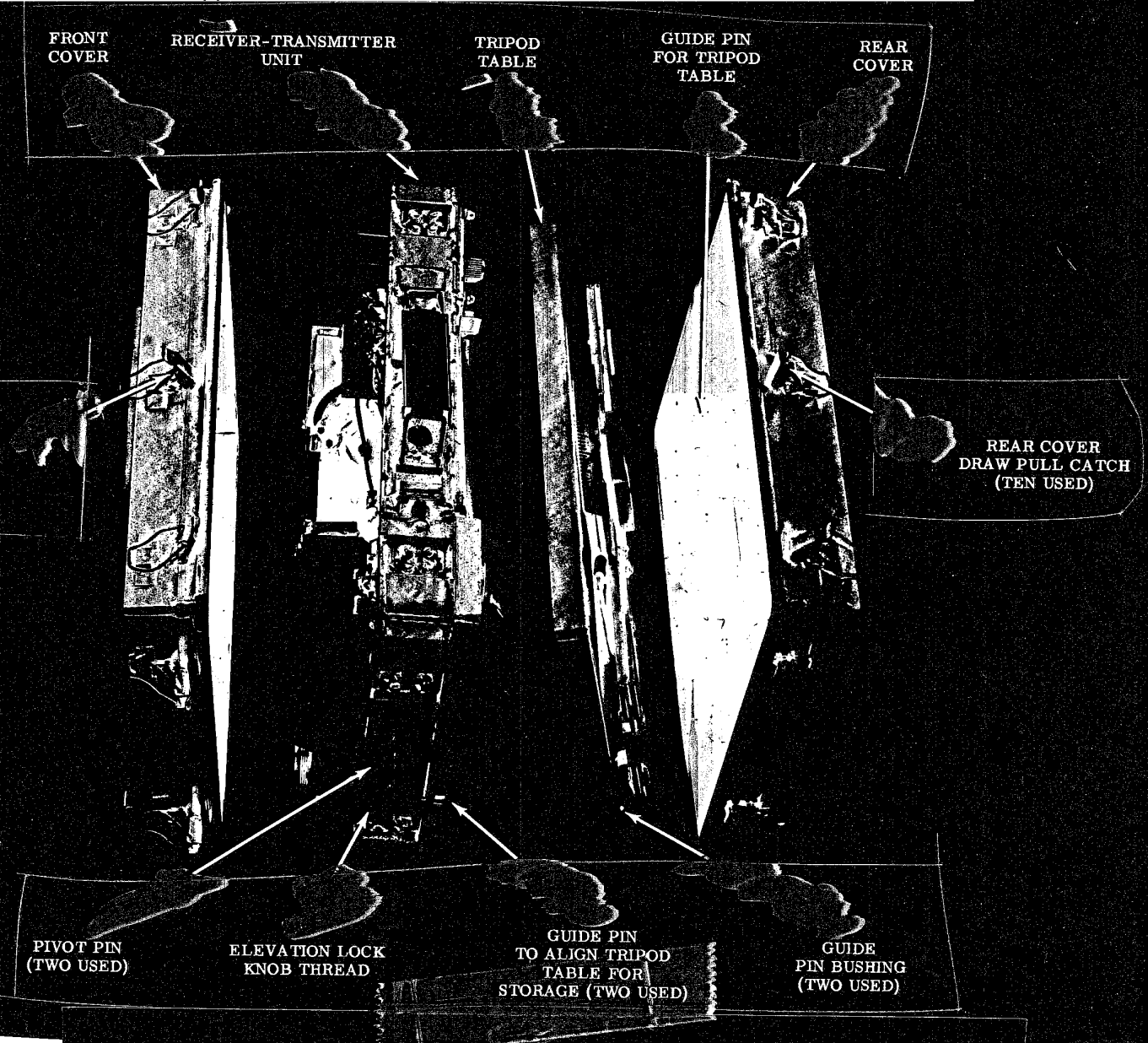
FIGURE 3-3. REAR VIEW OF INFRARED VOICE COMMUNICATOR PACKED FOR STORAGE BUT WITH REAR COVER AND TRIPOD TABLE REMOVED
