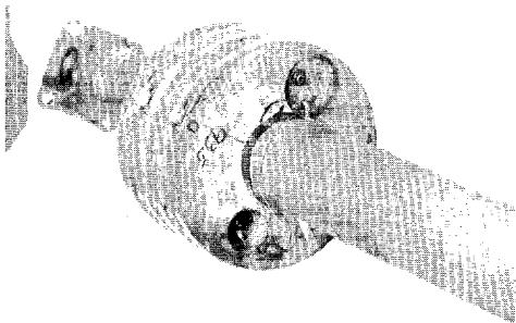
Drive Shaft 4 inches diameter. Instrumented for torque tests using T60 Transmitter.
