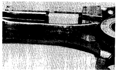
Subminiaturization of Transmitter permits mounting in confined areas with the transducer. Shown a Transmitter in the connecting rod of a diesel engine to measure temperature and strain during operation. Photo courtesy of General Electric Co.
