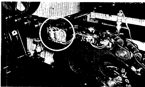
Application of subminiature T61 Transmitter for measurement of strain in links of a chain. Photo courtesy of Chain Belt Co.
