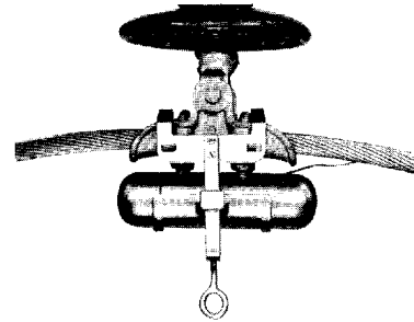
Transmitter in corona shield and weatherproof case for the measurement of vibratory strain and acceleration on high-voltage transmission lines to predict points of fatigue failure during high wind and icing conditions. Photo Courtesy of Preformed Line Products Co.
