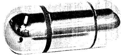
PORTEL 1 TO 3 CHANNEL TRANSMITTER WITH SUBCARRIER OSCILLATORS AND BATTERY IN CORONA-PROOF CASE FOR MEASUREMENTS IN HIGH VOLTAGE ELECTRICAL FIELDS. 10" Antenna
