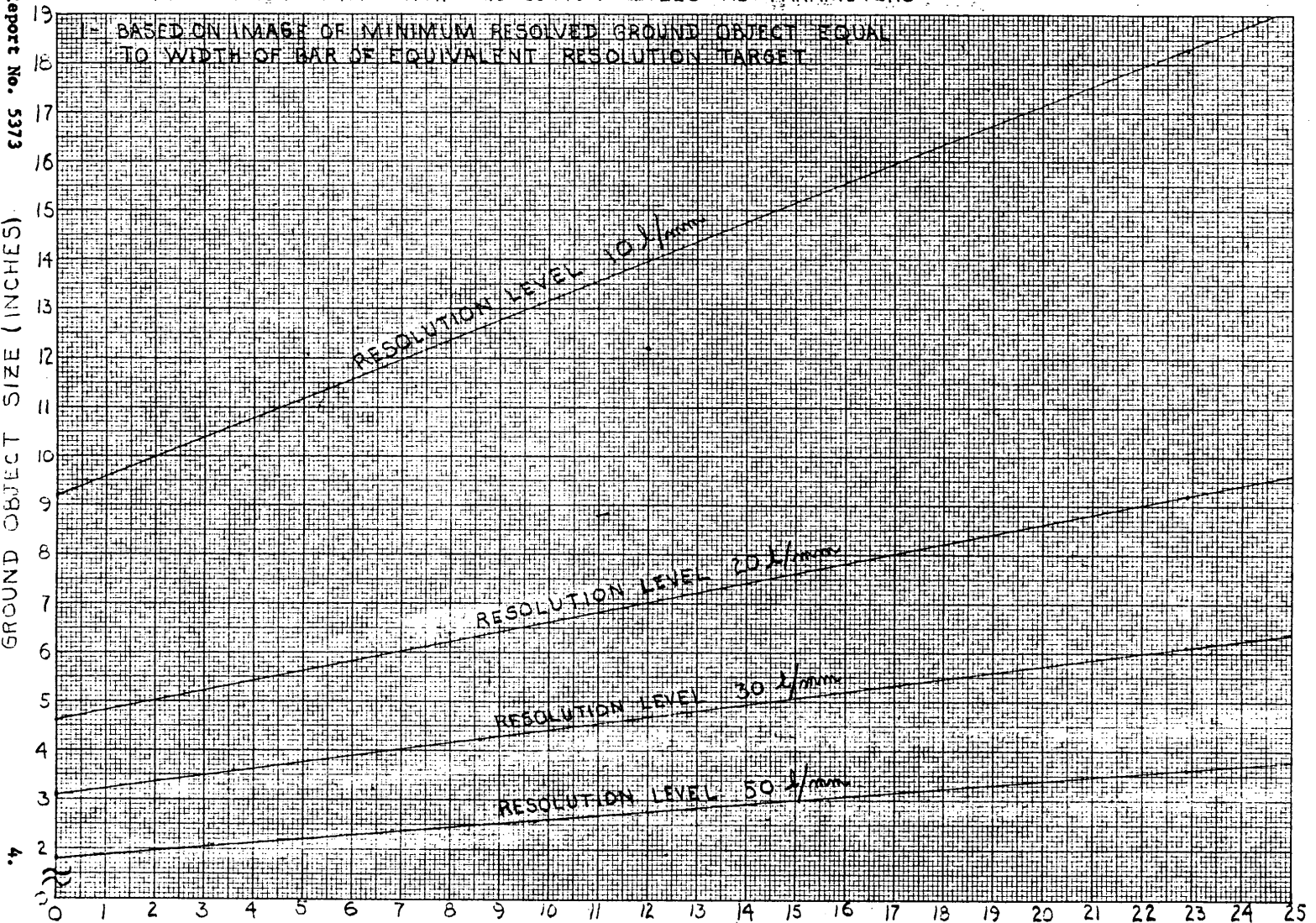
FIG. 1 - SIZE OF MINIMUM RESOLVED GROUND OBJECT AS A FUNCTION OF PERPENDICULAR DISTANCE FROM FLIGHT PATH WITH RESOLUTION LEVELS AS PARAMETERS
