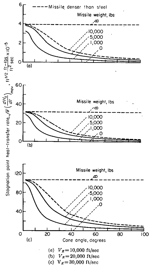
FIGURE 11.—Maximum rate of convective heat transfer to the stagnation point of spherically tipped cones of the same volume entering the earth's atmosphere at an angle of 30^\circ to the horizontal and velocities of 10,000, 20,000, and 30,000 ft/sec (volume = 16.34 cu ft).
