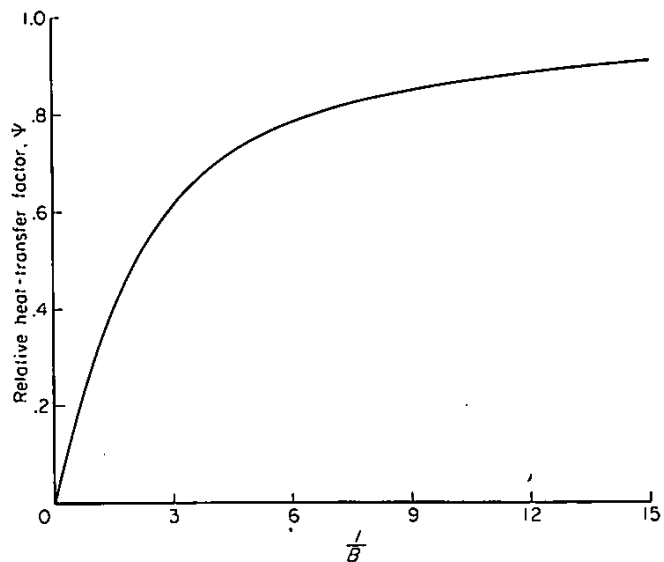
FIGURE 9.—Variation of relative heat-transfer factor \psi with 1/B .
