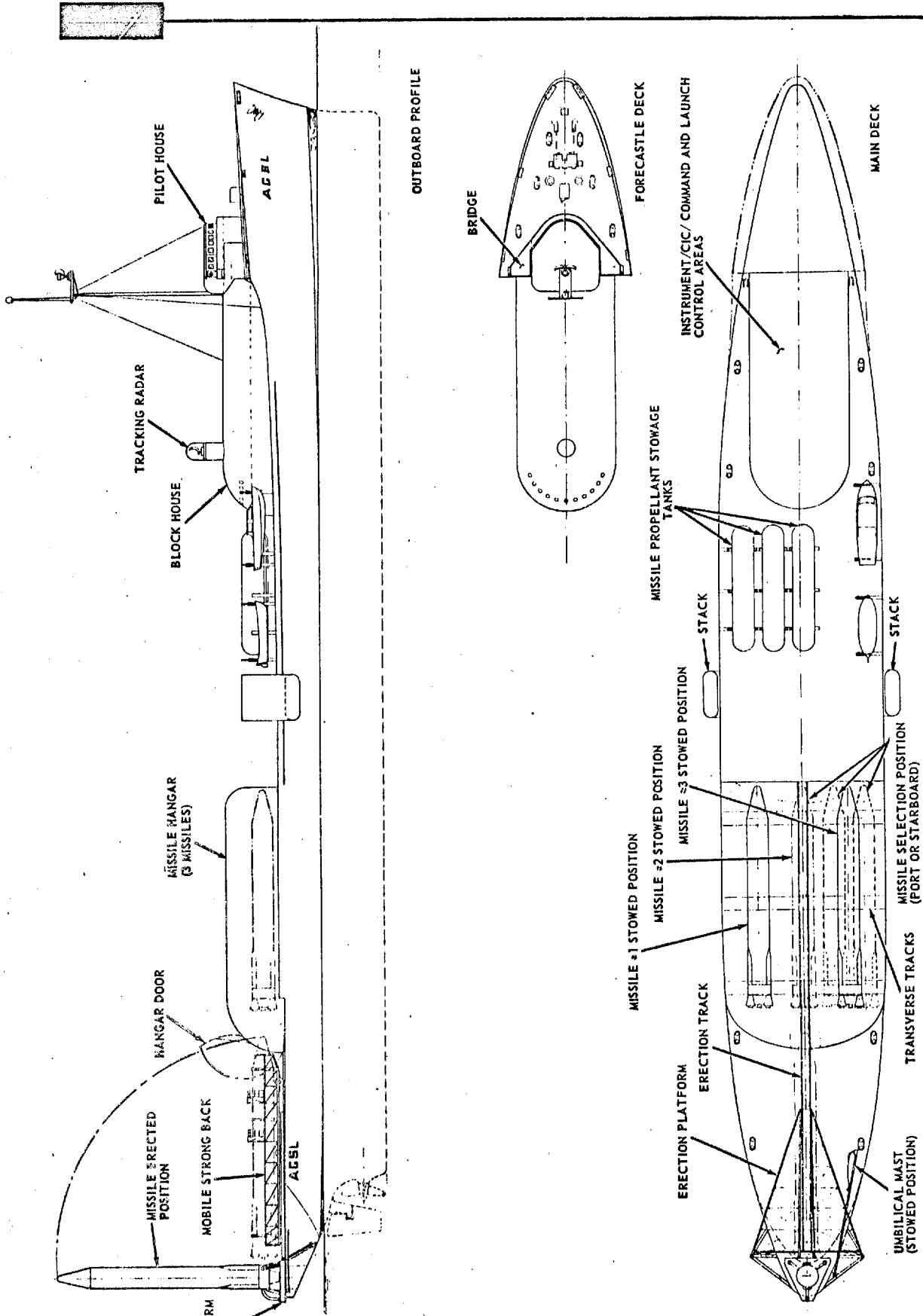
Figure 1 AGSL Mariner Outboard Profile
