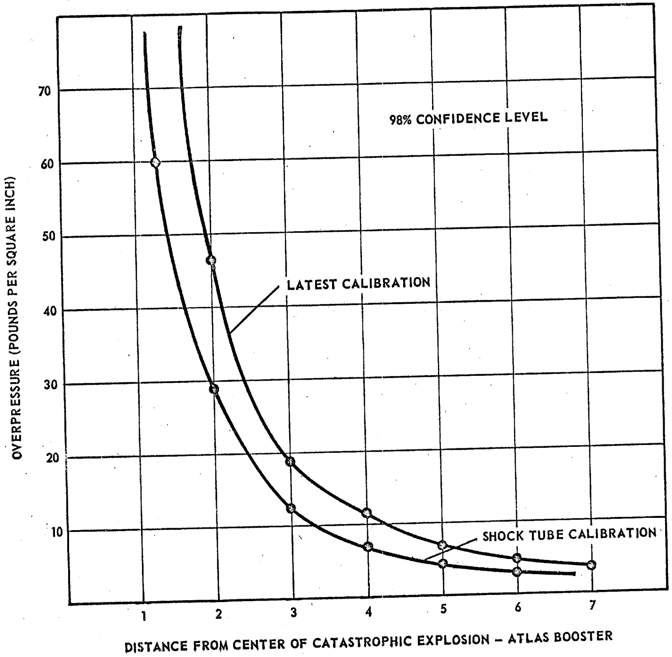
Figure 2 Overpressure vs Distance Based on Two Gage Calibrations for Atlas Tests
