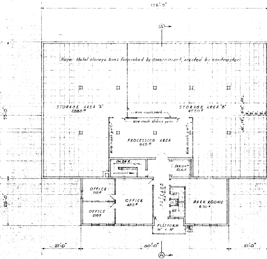
FIRST FLOOR PLAN - UPPER LEVEL
