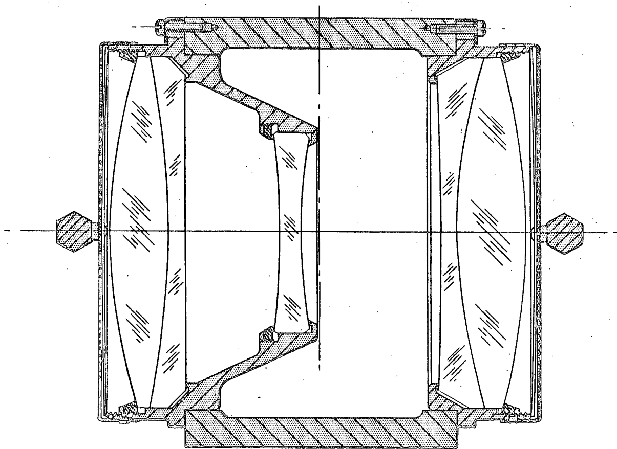
FIG. X. 24" f/8 LENS
