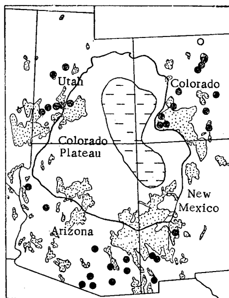
Fig. 3. Diagram of the location of uranium mineralization on the Colorado Plateau and in its surrounding terrain: 1) boundary of the Colorado Plateau; 2) effusive coverings; 3) region of development of sedimentary uranium deposits; 4) hydrothermal deposits and ore occurrences of uranium.
