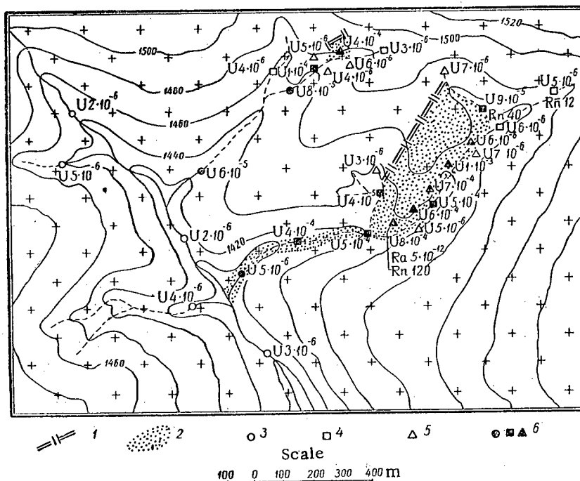
Fig. 7. Map of radiohydrogeological testing of different activities: 1) ore-bearing structure; 2) aureoles of anomalous waters of different concentration; 3) sites at which samples were taken from various springs and water courses; 4) boreholes sunk in the first stage of prospecting-surveying operations; 5) boreholes sunk in the second state of prospecting-surveying operations; 6) anomalous springs (the figures indicate anomalous contents of uranium and radium (g / liter) and radon (emanations)).
