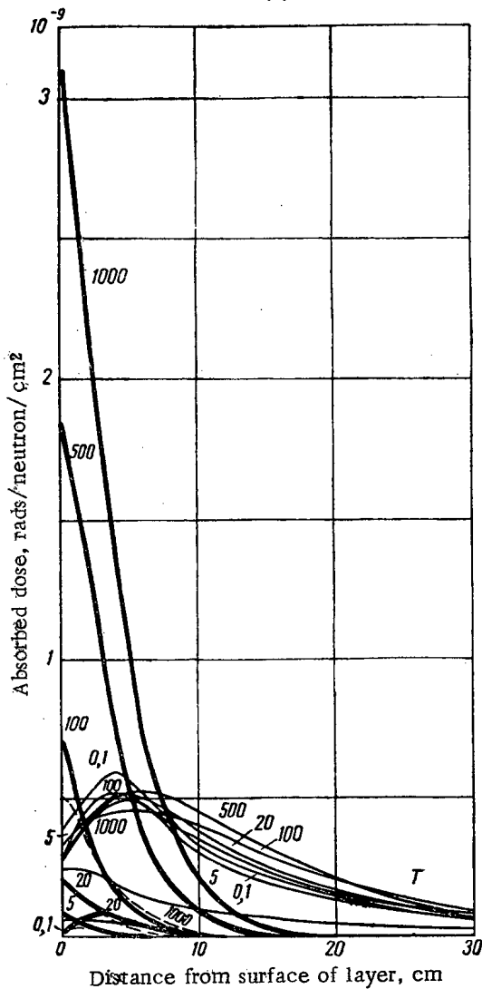
Fig. 1. Absorbed dose of a unit flux of neutrons incident perpendicularly on a tissue layer of thickness 30 cm [2]. The numbers on the curves represent the neutron energy in kiloelectron-volts; — recoil protons and protons from the reaction N(n, p) ; — \gamma rays from the reaction H(n, \gamma)D ; - - - heavy recoil nuclei.
