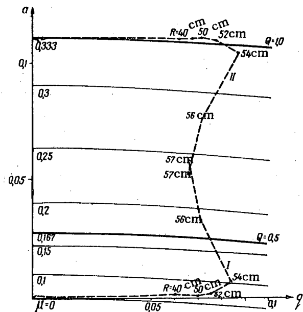
Fig. 2. Motion of the working points in the stability band. I) For vertical oscillations; II) for radial oscillations.
