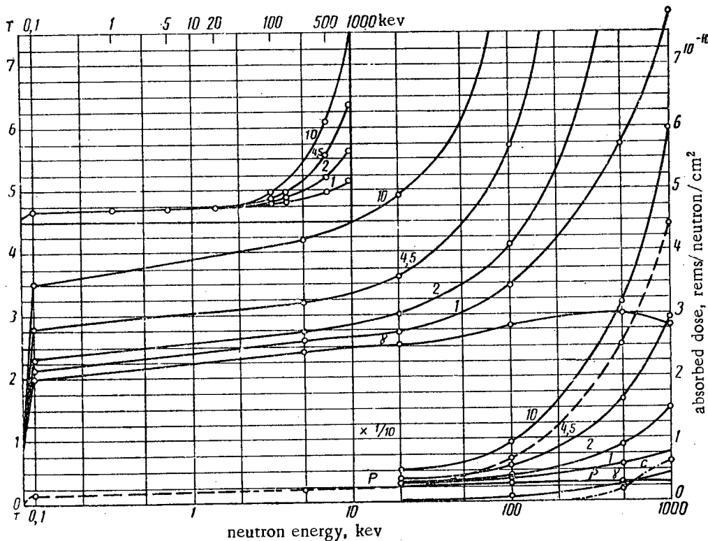
Fig. 3. Average-tissue absorbed dose for tissue layer irradiated by a unit neutron flux. The numbers on the curves represent the RBE values taken for protons. The absorbed dose of the individual components of secondary radiation is expressed in rads; \gamma - gamma radiation; p - protons; c - heavy recoil nuclei. The upper set of curves is normalized to the value at 1 keV.
