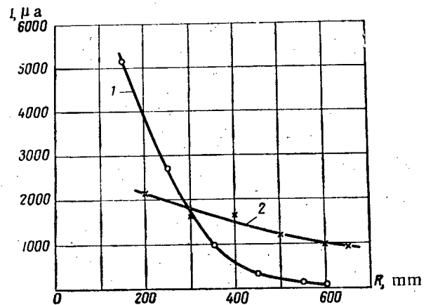
Fig. 8. Variation of the current with the radius at the probe position. 1) For an ordinary cyclotron; 2) for a cyclotron with an azimuthally varying magnetic field.
