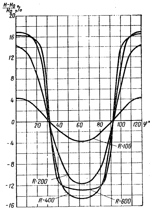
Fig. 6. Variation of the magnetic field intensity with the angle \varphi .
