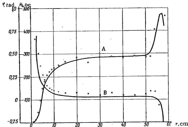
Fig. 6. A) Variation of the amplitude of the fourth harmonic of the magnetic field H_4 with the radius (solid curve - calculated, circles - experimental data); B) deviation of the phase of the fourth harmonic of the magnetic field from a spiral (solid curve - calculated; crosses - experimental data).
