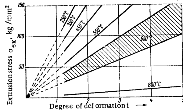
Fig. 8. Nomogram for determining extrusion stresses.
