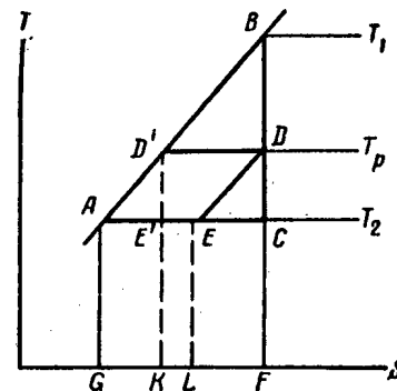
Fig. 4. T-S diagram of cycle of boiling liquid with regeneration.
