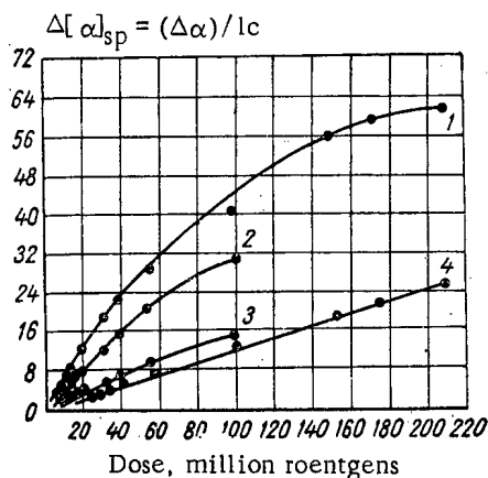
Fig. 3. Variation in angle of rotation of plane of polarization of sucrose solutions as a function of irradiation dose (in percent): 1) 5; 2) 10; 3) 30; 4) 45.
