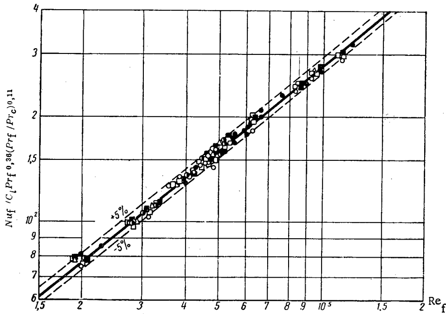
Fig. 3. Generalized dependence of the mean values of the heat-transfer coefficient on Re_f . The experimental points are characterized by the following values of the ratio l/d : ○) 1.5; □) 3.0; △) 7.5; ●) 15; ■) 22.5; ●) 80.
