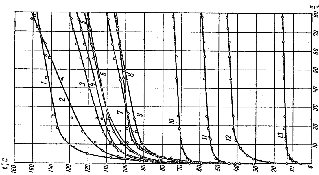
Fig. 1. Distribution of wall temperature in the tube ( q in kcal/m 2 · hr):
