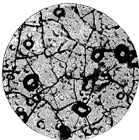
Fig. 1. Layer of uranium compound of density 1 mg/cm 2 (× 600).
