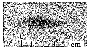
Fig. 13. Photograph of beam obtained by placing a copper plate irradiated by deuterons on photographic emulsion.
