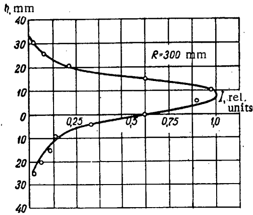
Fig. 9. Vertical distribution of the ion beam intensity.
