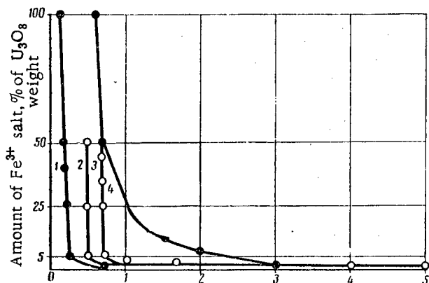
Fig. 1. Relation between the uranium solution time and the amount of \text{Fe}^{3+} salt added in the solution of uranous-uric oxide in solutions of nitric and sulfuric acids with \text{MnO}_2 and 100% solution of the oxide at t = 90^\circ\text{C} . 1, 4) Nitric acid (50 and 5 g/liter, respectively); 2, 3) sulfuric acid (5 and 150 g/liter, respectively).
