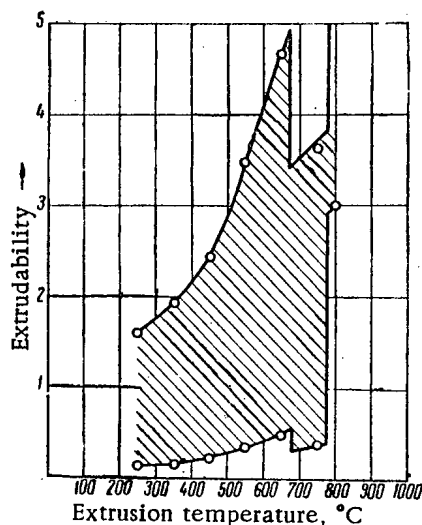
Fig. 10. Relationship between extrudability of uranium and the temperature.
