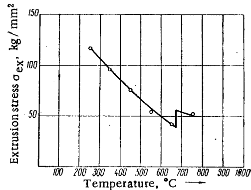
Fig. 6. Relationship between the extrusion stress for uranium and the temperature.
