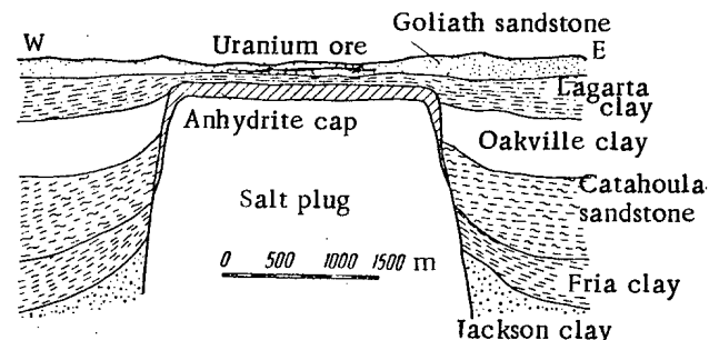
Fig.5. Diagram of the position of uranium mineralization in the petroleum structure in the Panhandle, Texas.
