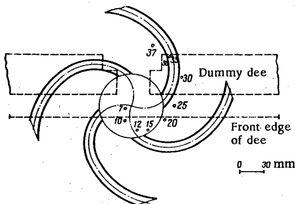
Fig. 1. Position of the centers of instantaneous orbits for N = 4 .
