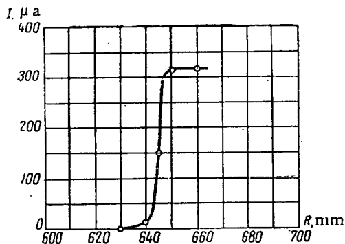
Fig. 11. Absorption curve taken with an aluminum filter.
