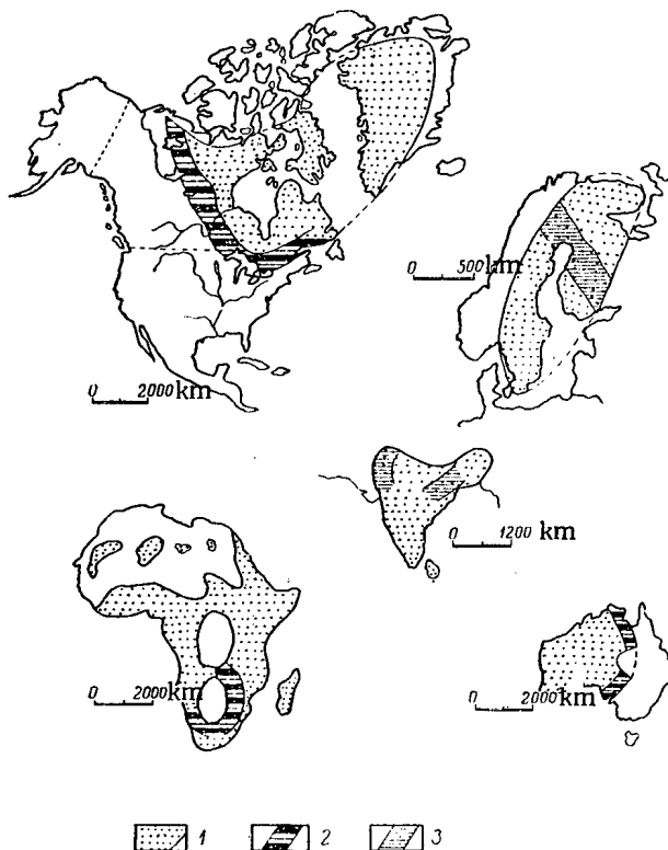
Fig. 1. Location of uranium-bearing belts in Precambrian shields: 1) Precambrian shields; 2) ore belts with large uranium deposits; 3) ore belts with slight uranium mineralization.
