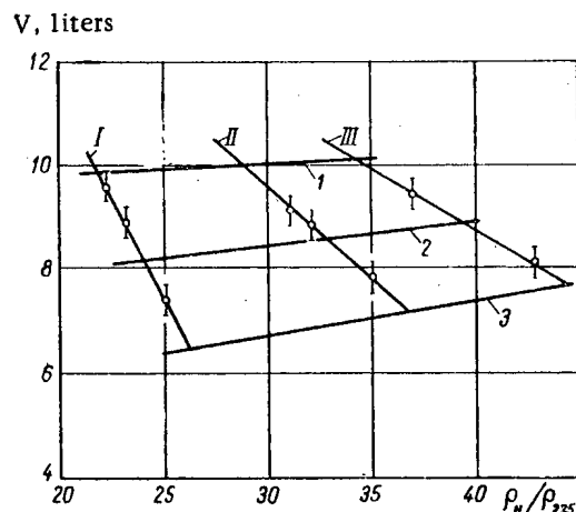
Fig. 5. Dependence of critical dimensions of uranium-water system on ratio \rho_H/\rho_{235} for different water densities: 1, 2, 3) water density \gamma equal to 0.8, 0.9, 1.0 g/cm 3 , resp.; I, II, III) U 235 concentrations equal to 836, 627, 523 g/liter, resp.
