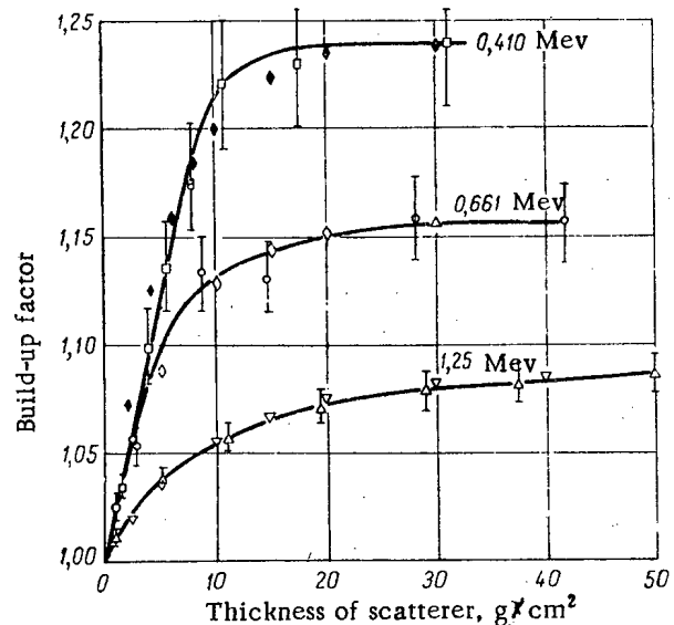
Fig. 3. Dependence of the value of the energy build-up factor on the thickness of the scattering material: □, ○, △) experimental points; ◆, ◇, ▽) calculated points (12).
