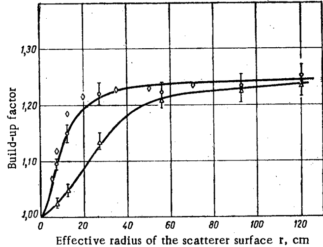
Fig. 2. The dependence of the value of the reflection energy build-up factor for Au 198 γ rays on the size of the scattering surface: ○, △) experimental points (h is 1.1 and 12.5 cm, respectively); ◇) calculated points [h = 1.1 cm (11)].
