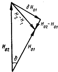
Fig. 1. Diagram of phase and amplitude inhomogeneities of the magnetic field.
