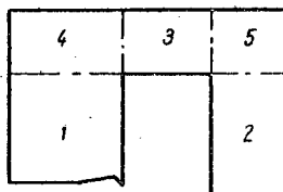
Fig. 7. Arrangement of segments in stock metal for a four-yoke electromagnet, prior to machining.
