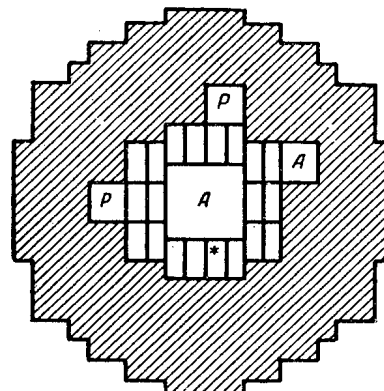
Fig. 1. Diagram of annular uranium-water system, with graphite lateral reflector ( \rho_H/\rho_{235} = 31 ): The blank rectangles are working cells, while the hatched area is the graphite; P are control rods; A are scram rods; * indicates a movable cell.
