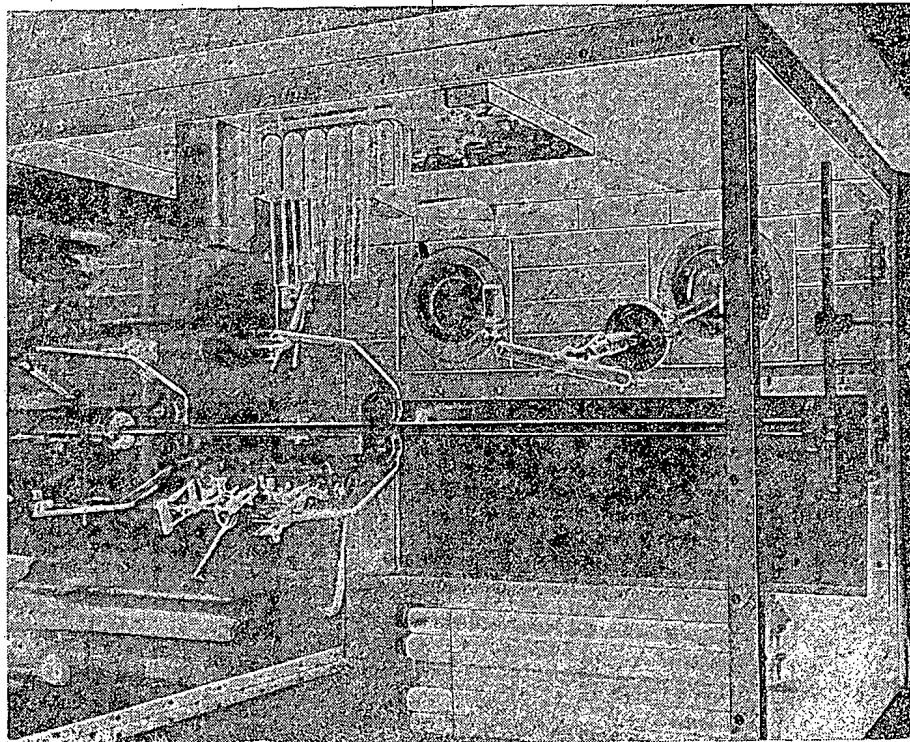
Fig. 2. Hot-cell with manipulator.
