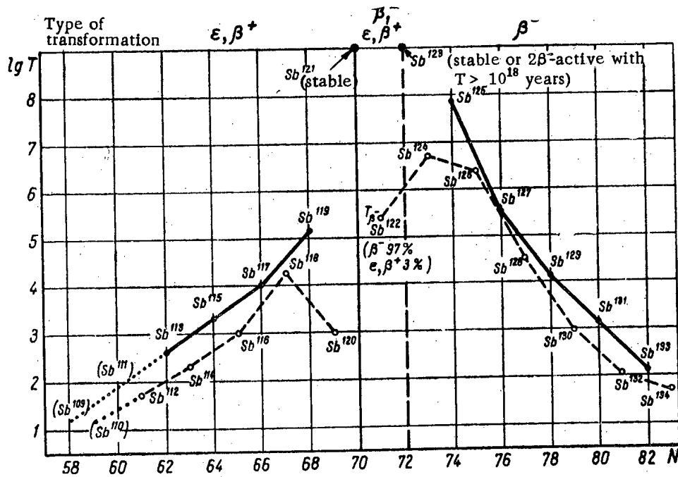
Fig. 3. Half-lives of radioactive isotopes of antimony. Neutron number N is plotted on the abscissa. The left branch of the curve corresponds to \epsilon - and \beta^+ - active isotopes, and the right branch corresponds to \beta^- - active isotopes. As yet undiscovered isotopes are indicated in parentheses.
