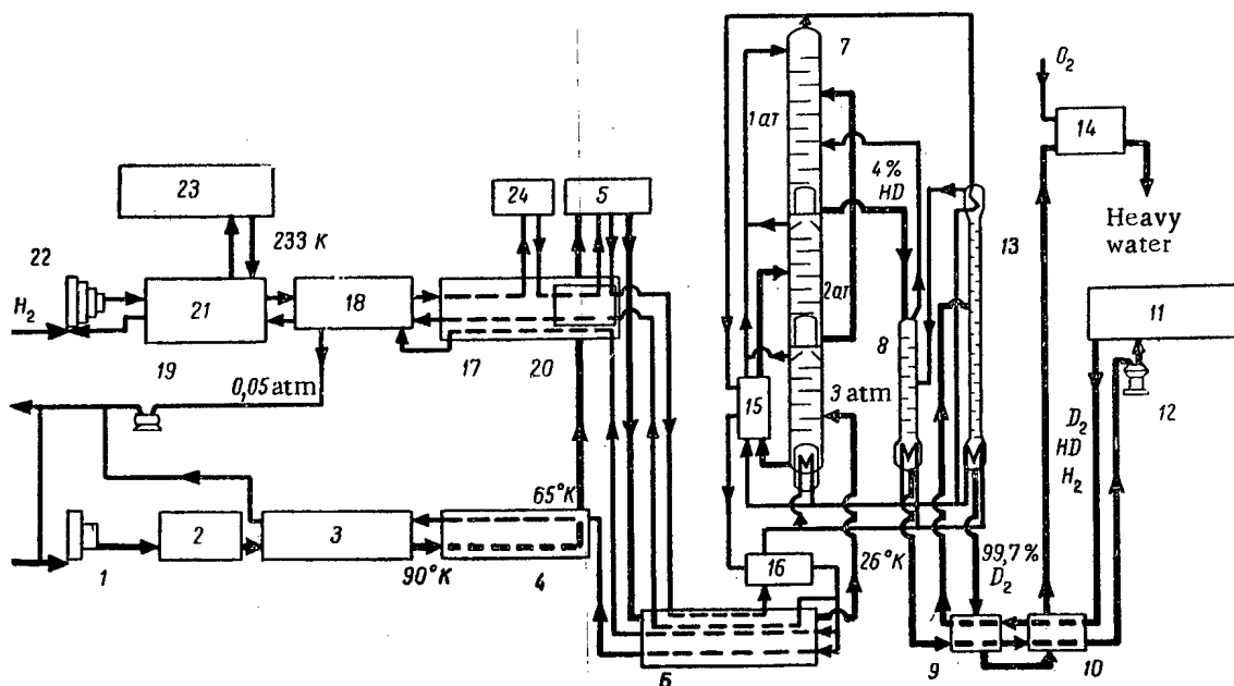
Flowscheme of production of heavy water by the low-temperature distillation method.
