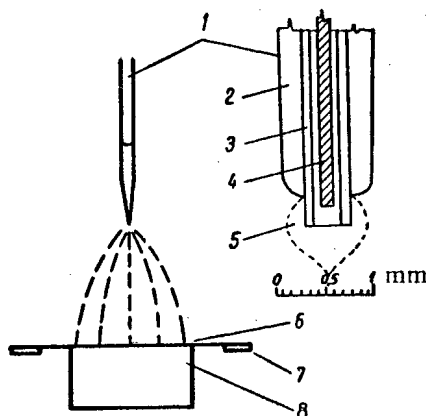
Method of layer deposition: 1) Glass capillary 0.4 to 0.5 mm in diameter; 2) paraffin; 3) capillary; 4) tungsten; 5) conical solution drop; 6) organic film; 7) aluminum ring; 8) aluminum support.
