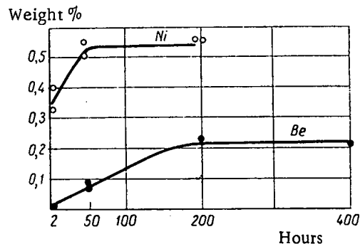
Fig. 4. Kinetics of the dissolution of nickel in lithium at 750^{\circ}\text{C} and beryllium at 1000^{\circ}\text{C} .
