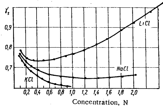
Fig. 3. Dependence of the activity coefficients of alkali metal chlorides upon the concentrations of their solutions.
