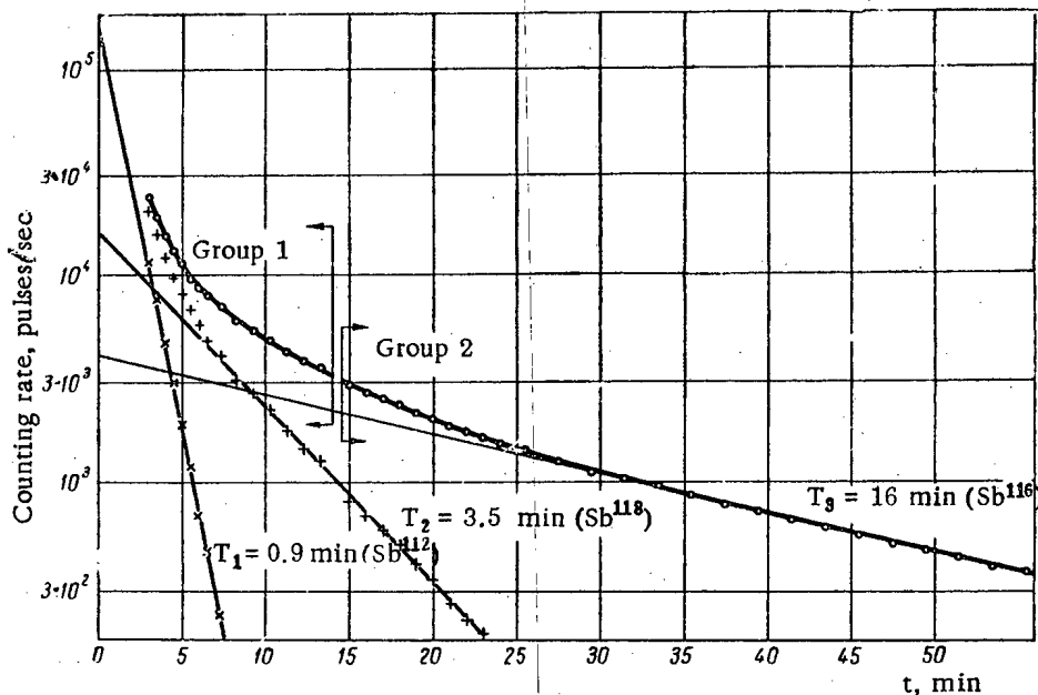
Fig. 1. Half-lives of radioactive isotopes of antimony chemically separated from tin enriched with Sn^{112} , after irradiation of the tin by protons.
