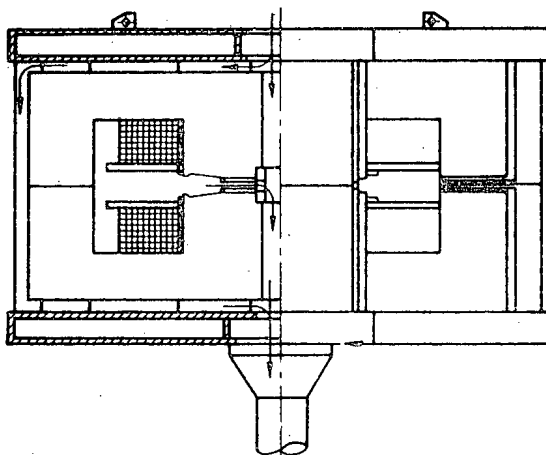
Fig. 8. Path of cooling air in electromagnet.
