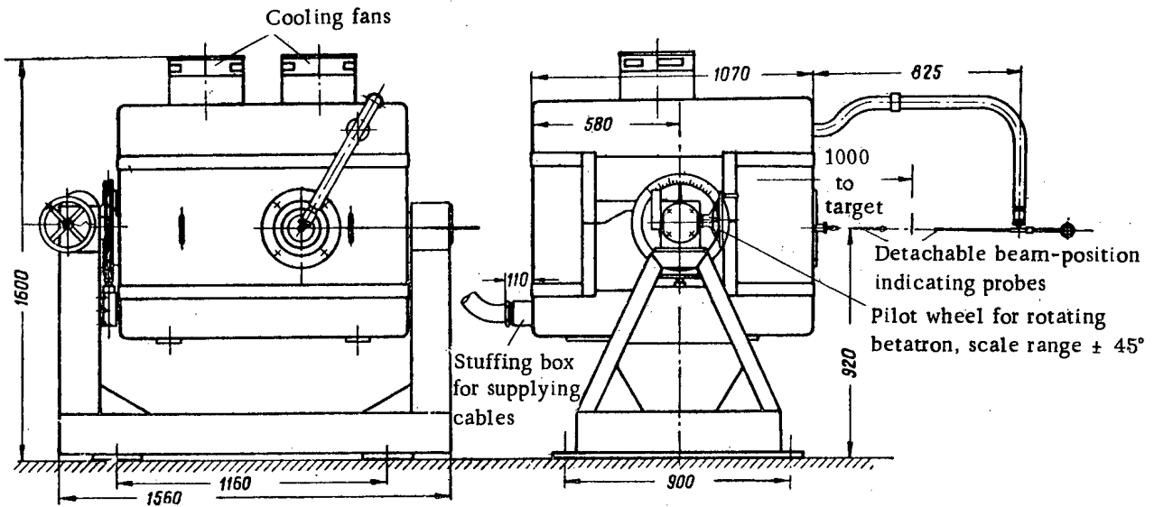
Fig. 11. Rotating 25 Mev betatron, for nondestructive testing.
