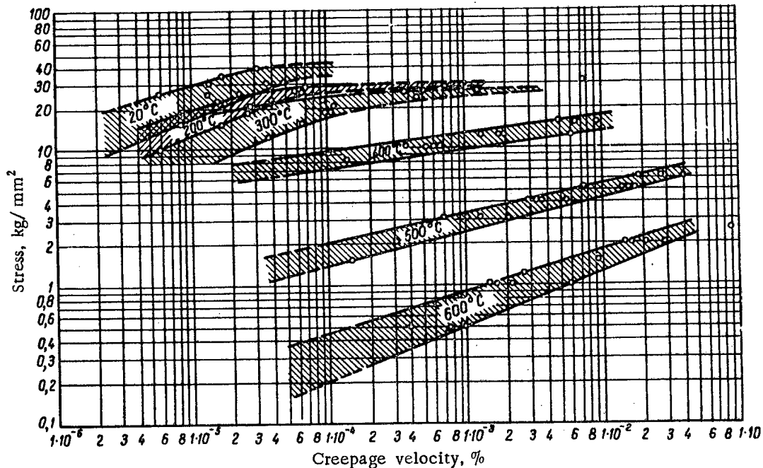
Fig. 2. Change in the creep rate of hot rolled uranium in relation to the temperature and stress.
