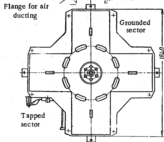
Fig. 9. Stationary 4-yoke betatron, 20 Mev.
