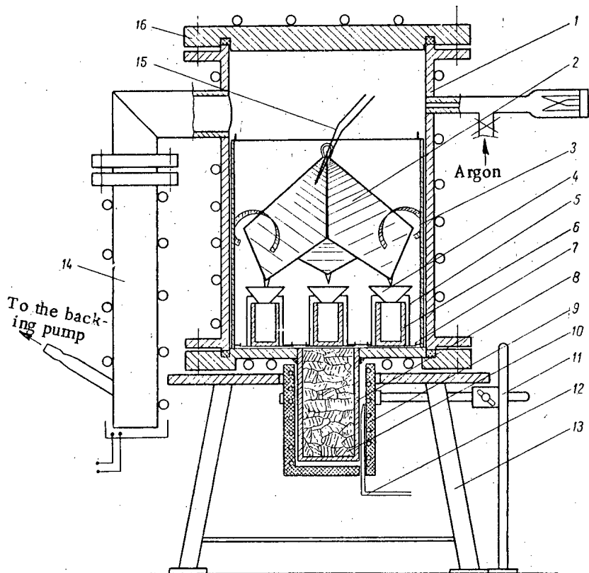
Fig. 1. Diagram of the apparatus for filling crucibles with distilled lithium: 3) screen on which sodium and potassium condense; 4) funnel; 5) screen; 7) backing; 11) support; 12) thermocouple; 13) brace; 14) diffusion pump; 15) thermocouple; 16) cover (remainder of the legend given in the text).
