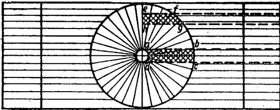
Fig. 4. Arrangement of steel laminations in a two-yoke electromagnet.
