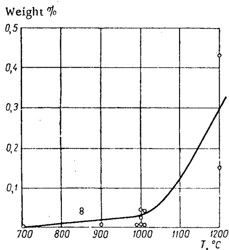
Fig. 5. Solubility of zirconium in lithium at 700-1000°C.
