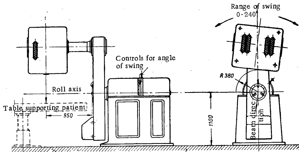
Fig. 13. Pendulum-type tiltable betatron, 15 Mev, for medical applications.
