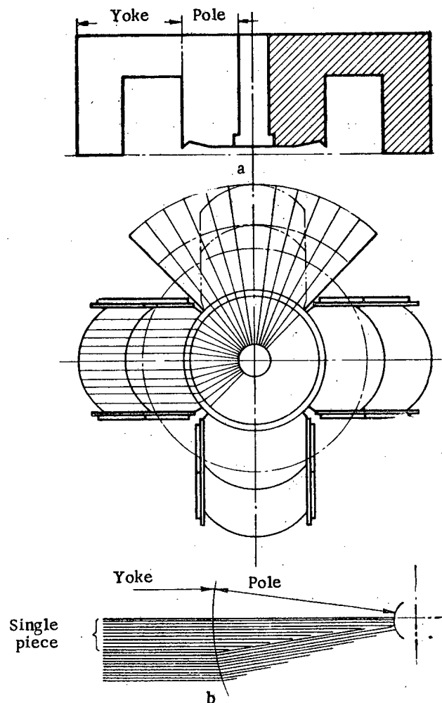
Fig. 2. Diagram of 4-yoke design of magnetic leads to betatron.
