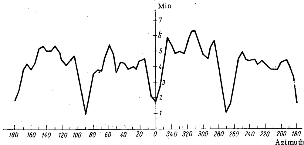
Fig. 3. Azimuthal phase variation of the magnetic field across the gap of a 4-yoke electromagnet.
