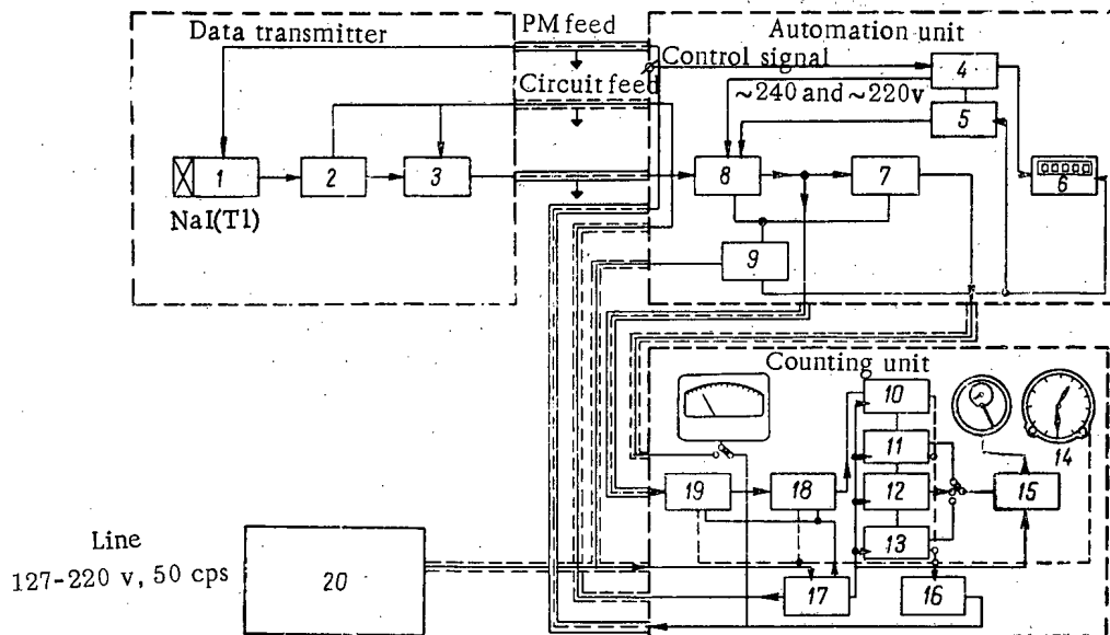
Fig. 1. Schematic diagram of the RSU device. 1) Photomultiplier; 2) multivibrator; 3) cathode follower; 4) automatic control circuit; 5) time relay; 6) electric clock; 7) intensity meter; 8) input stage; 9) feed unit; 10-13) scaling circuits; 14) clock; 15) EMS stage; 16) high-voltage feed units; 17) feed units; 18) scaling circuit; 19) input stage; 20) SNE-220-05 stabilizer.
