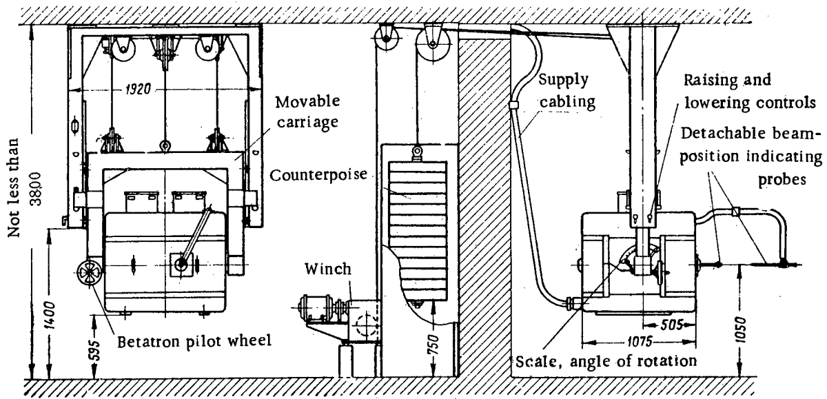
Fig. 10. Ceiling-suspended rotary betatron, 25 Mev, for medical applications.
