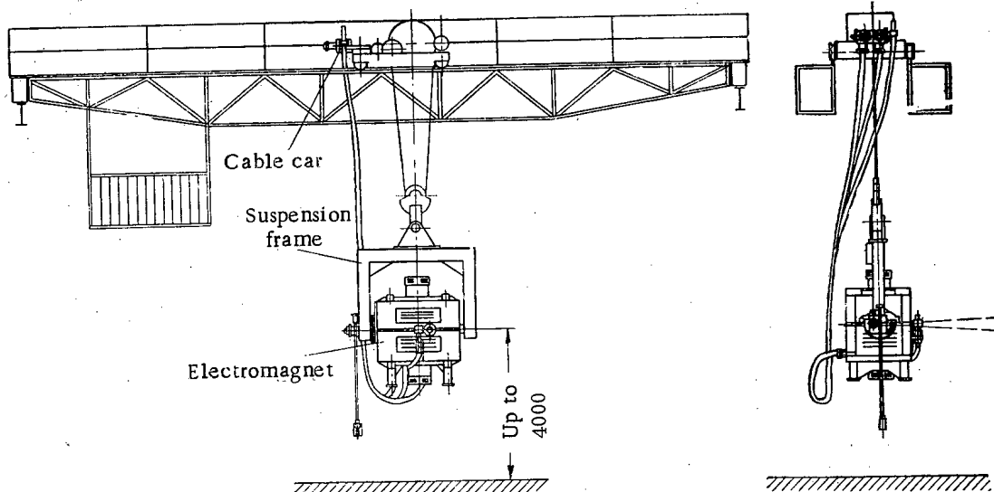
Fig. 12. Crane-suspended 25 Mev betatron, for nondestructive testing.
