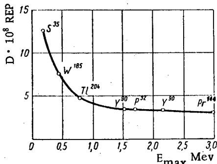
Fig. 3. Relation between size of dose D_1 for one \beta particle and maximum energy of the \beta spectrum.
