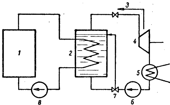
Fig. 1. Schematic diagram of the plant. 1) Reactor; 2) steam generator; 3) throttle; 4) turbine; 5) condenser; 6) second loop pump; 7) valve; 8) first loop pump.
