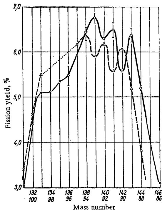
Yield-mass curve for fragments from U^{235} fission.
