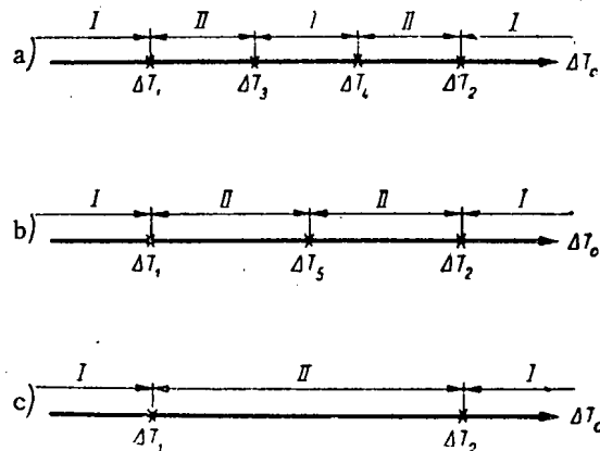
Fig. 4. Stability regions of the plant for \delta < 0 . a) B^2 - 4AC > 0 ; b) B^2 - 4AC = 0 ; c) B^2 - 4AC < 0 ; I) instability region; II) stability region. (At the points \Delta T_1 , \Delta T_2 , \Delta T_3 , \Delta T_4 , and \Delta T_5 , the system is unstable.)
