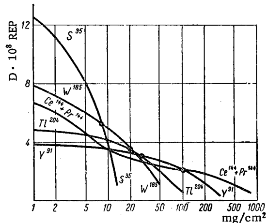
Fig. 4. Deep doses in the field of S^{35} , W^{185} , Tl^{204} , Y^{91} , and Ce^{144} + Pr^{144} sources.
