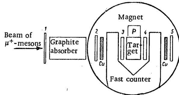
Diagram of experimental arrangement for determining the g -factor of a \mu -meson (numerical figures denote scintillation counter units), with P as the specimen for measuring nuclear magnetic resonance effects.
