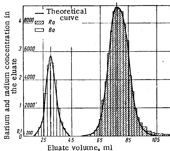
Fig. 3. Theoretical and experimental data on the elution of barium and radium.
