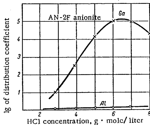
Fig. 7. Relation of the distribution coefficient of gallium to hydrochloric acid concentration.
