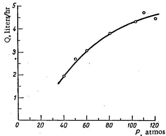
Fig. 5. Curve showing the dependence of liquefier capacity on pressure.
