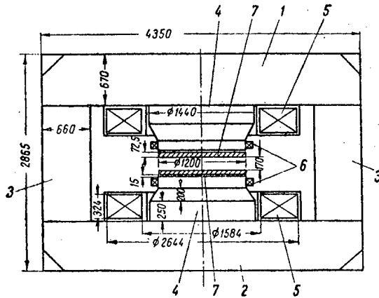
Fig. 2. Schematic diagram of the magnet. 1) upper cross piece; 2) lower cross piece; 3) vertical post; 4) pole pieces; 5) main winding; 6) auxiliary winding; 7) roof of the acceleration chamber.
