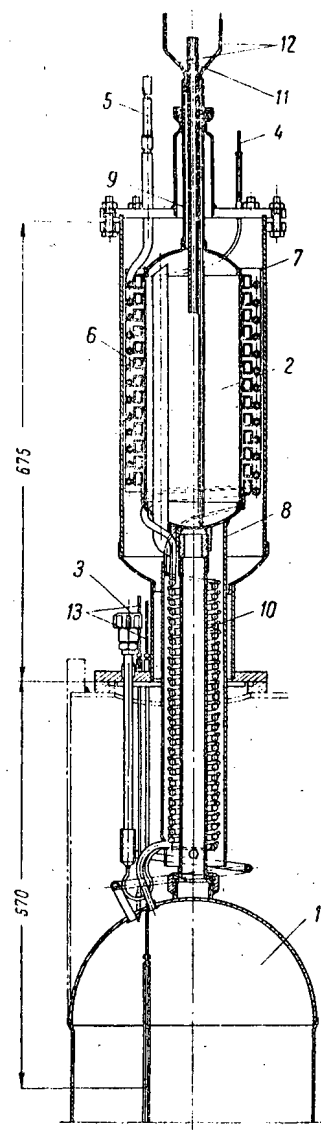
Fig. 2. Section of the hydrogen liquefier.
