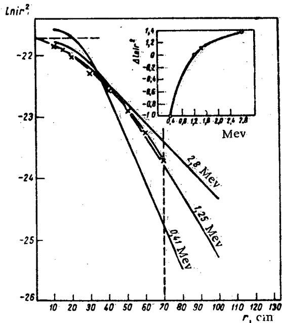
Fig. 4. Spatial distribution of \gamma radiation: — data from [7] for \gamma radiation in water; *— data for \gamma radiation of the fragments in water according to (1) for t = 1 sec; --- data for \gamma radiation of the fragments in air for t = 1 sec.
