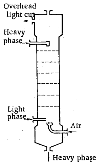
Fig. 1. Diagram of a tray tower with air mixing.
