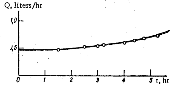
Fig. 4. Curve showing the dependence of hydrogen consumption on time under conditions of strong outgassing. The operating pressure is 1.4-1.2 \cdot 10^{-6} mm Hg.
