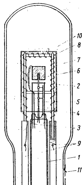
Electron-radiation calorimeter.
