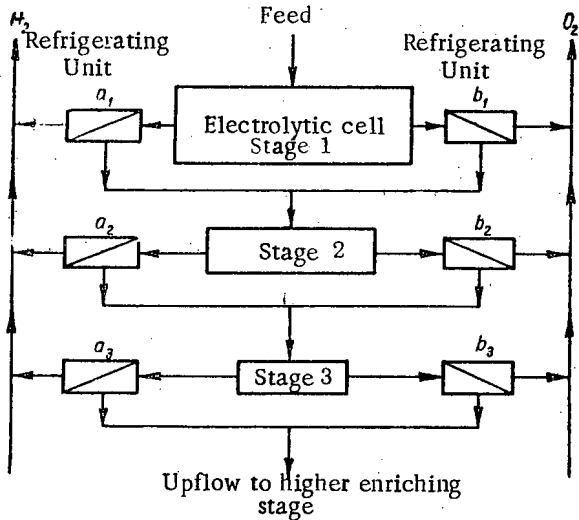
Fig. 1. Flowsheet of electrolytic production of heavy water.
