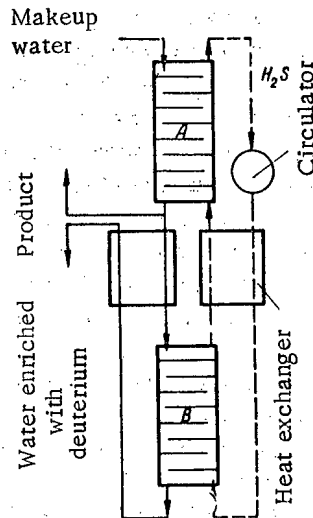
Fig. 3. Flow scheme of a "dual-temperature" exchange process.
