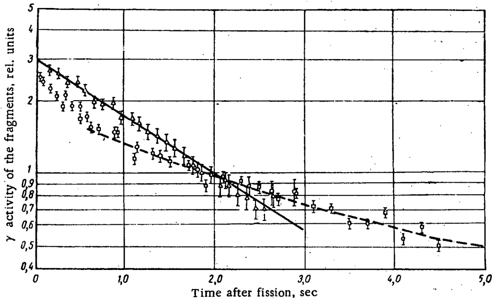
Fig. 1. Kinetics of the short-lived \gamma radiation of the U^{235} fission fragments: ---- data of the present study; \circ - data of I. I. Levintov and V. N. Shamskev; \triangle - data of [4]; \square - data of O. I. Leipunskii and co-workers for the fission of natural uranium by 14 Mev neutrons.
