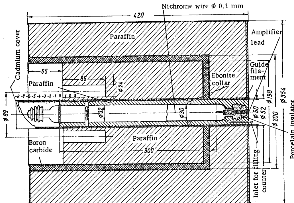
Fig. 1. Diagram of the neutron detector.
