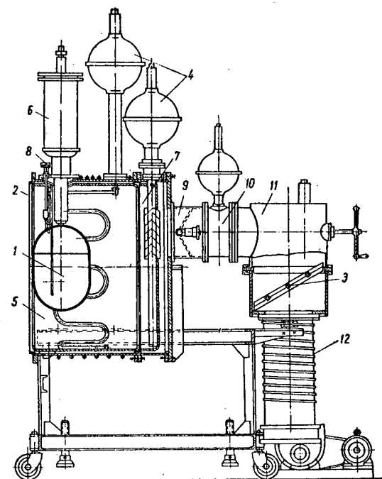
Fig. 1. Diagram of the hydrogen condensation pump.
