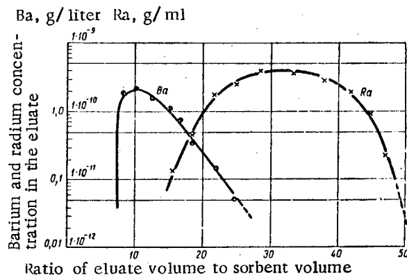
Fig. 2. Barium and radium separation with hydrochloric acid elution.
