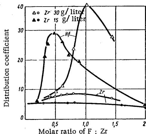
Fig. 5. Relation of distribution coefficients of zirconium and hafnium to the fluorine ion concentration for a solution containing 0.65 M sulfuric acid.
