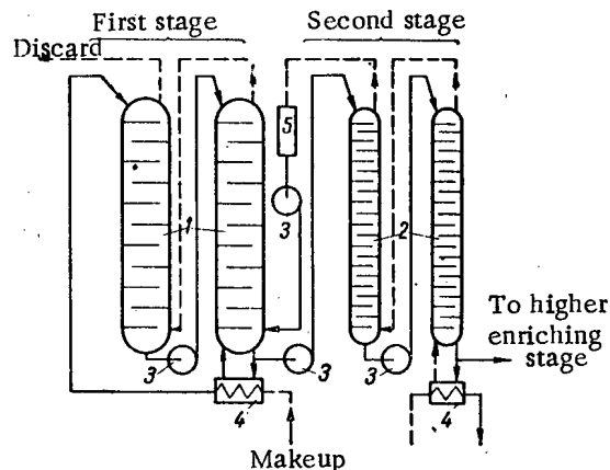
Fig. 4. Flowsheet of facility for extracting heavy water by the water-distillation method.
