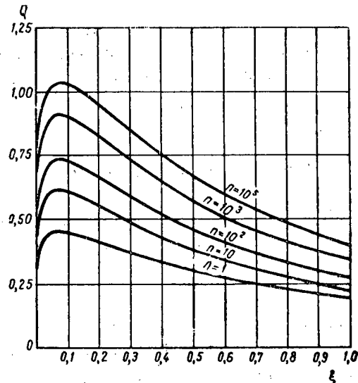
Fig. 2. Graph of the Q(xi) function for different numbers of cycles n.
