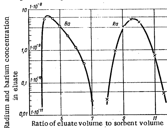
Fig. 4. Barium and radium separation with ammonium citrate.
