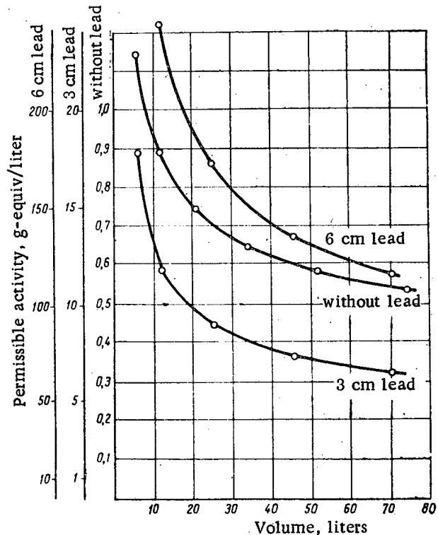
Fig. 3. Dependence of limiting permissible concentrations of gamma-active substances on volume of the solution for various thicknesses of lead shielding.
