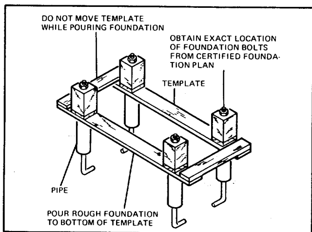
Figure 2. Template Used for Locating Foundation Bolts
