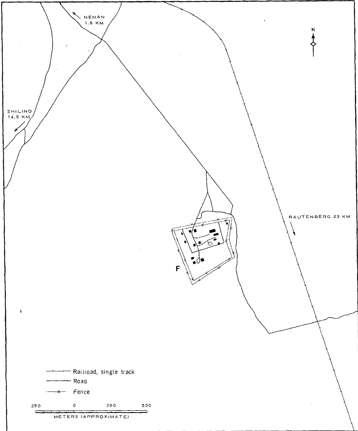
FIGURE 3. EXPLOSIVES STORAGE DEPOT. Sketch compiled from [redacted] NPIC J-4934 (11/64) June 1964.
